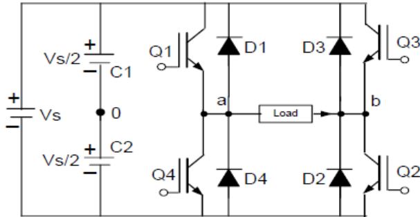
Gambar 1. Full Brige 1-Phase Inverter
